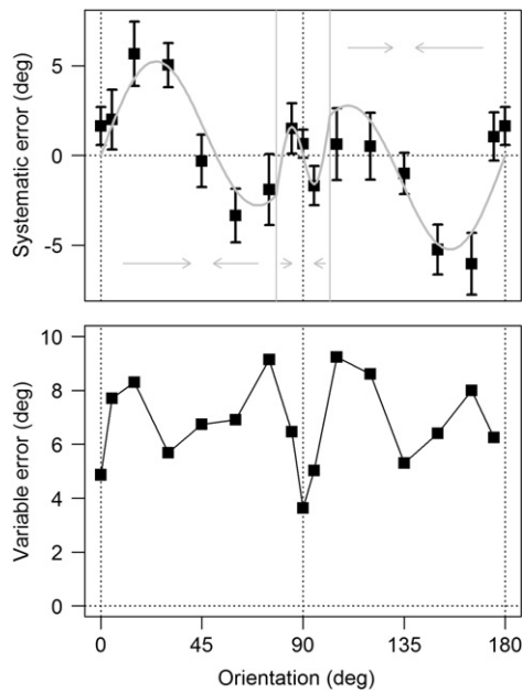
Fig. 1. Orientation-dependent error patterns. Top: average systematic error (solid squares) for each tested orientation (all responses from all participants are pooled together at each orientation). A positive error corresponds to a clockwise rotation while a negative error corresponds to a counterclockwise rotation. Vertical error bars correspond to 90% confidence intervals. The arrows indicate the direction of the bias and the gray line represents the prediction of the descriptive model (Eq. 5). Bottom: variability of the responses for each orientation (standard deviation of all responses from all participants).
