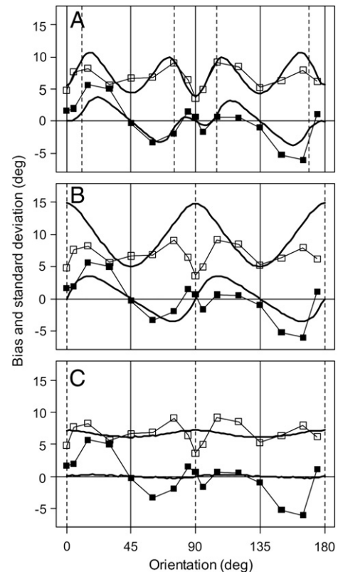
Fig. 2. CA model predictions. A: predictions of the extended CA model including the vertical and horizontal categories in addition of the oblique categories fitted to predict both the bias and the variable error by minimizing the MSE. B: original model CA including only the oblique categories fitted to predict the bias. C: original model fitted by minimizing MSE. For all panels, the solid and empty squares denote the average and standard deviation of the participants' responses respectively. The thick lines denote the model predictions. The vertical lines correspond to the prototypes (dotted lines) and category boundaries (solid lines).
